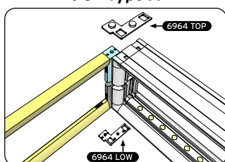
90° Type A
